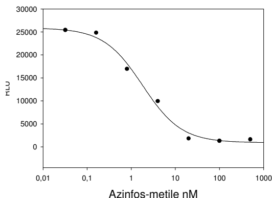
Fig.1. A typical competitive curve for Azinphos-methyl.
