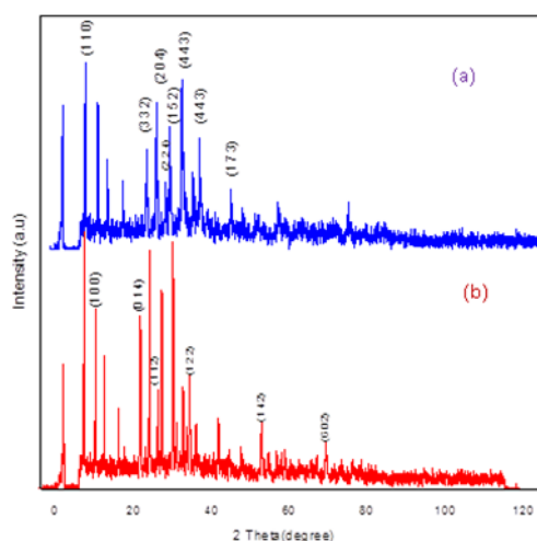
Figure 2. XRD patterns of (a) zeolite Y (b) copper loaded zeolite catalyst.
