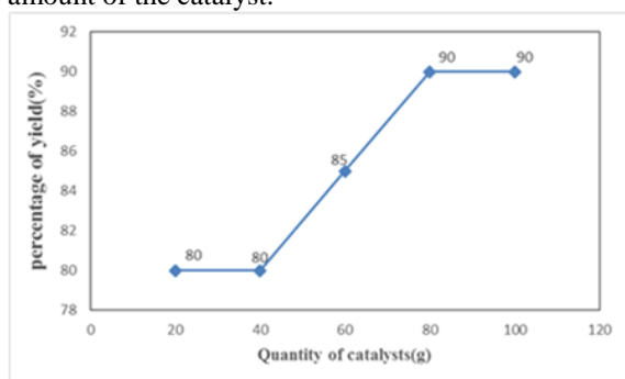
Figure 3. Effect of catalyst loading.
