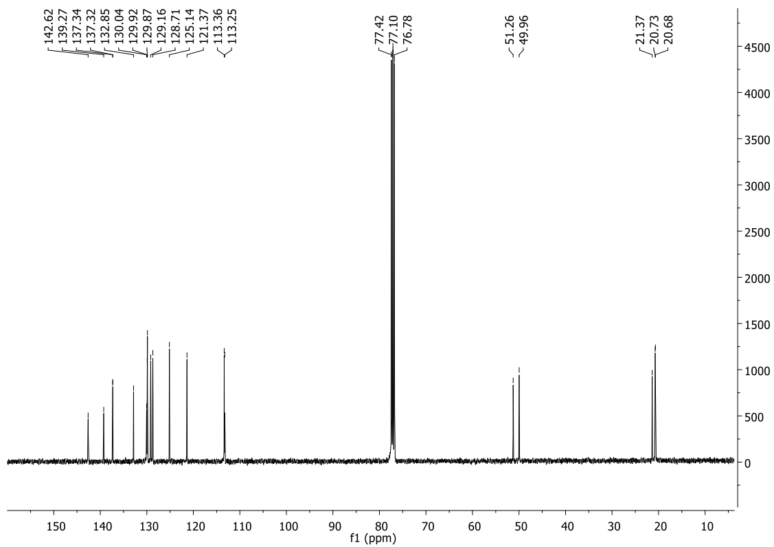
Figure S3. ^1\text{H} and ^{13}\text{C}\{^1\text{H}\} NMR spectrums of 2
