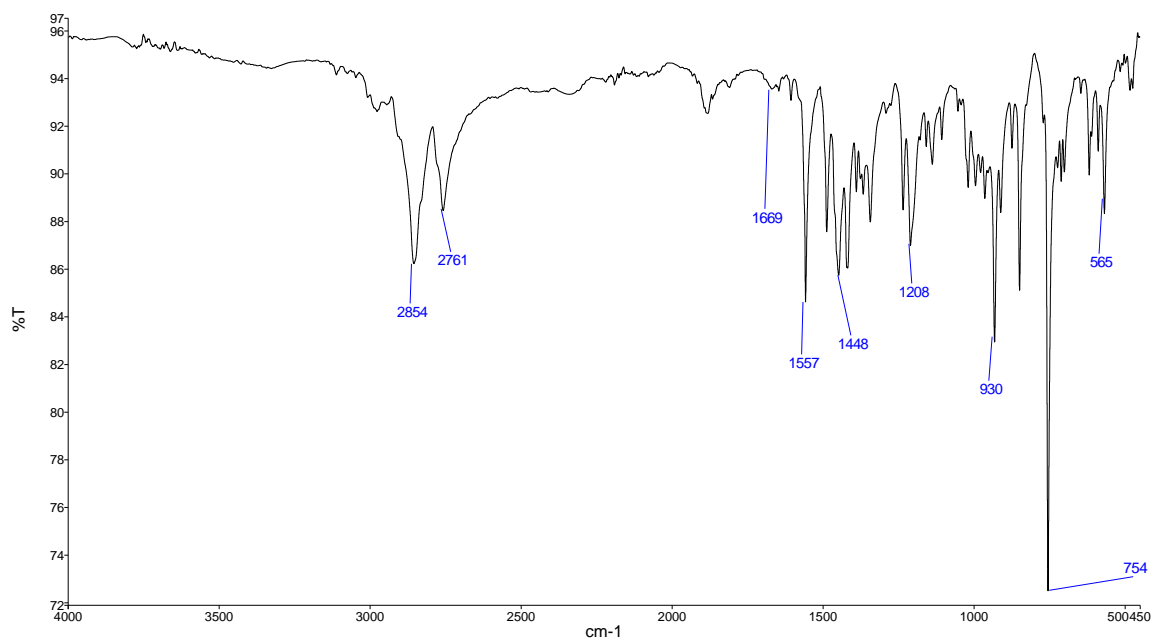
Figure S2. FT-IR spectrum of 1
