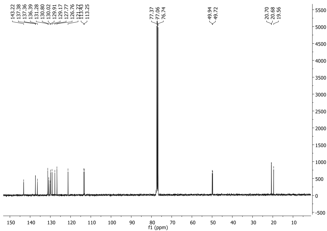
Figure S1. ^1\text{H} and ^{13}\text{C} NMR spectra of 1
