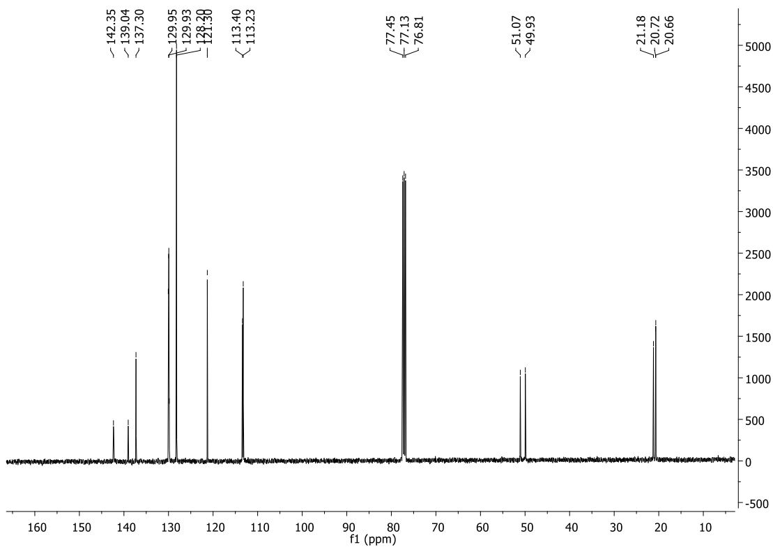
Figure S5. ^1\text{H} and ^{13}\text{C}\{^1\text{H}\} NMR spectra of 3
