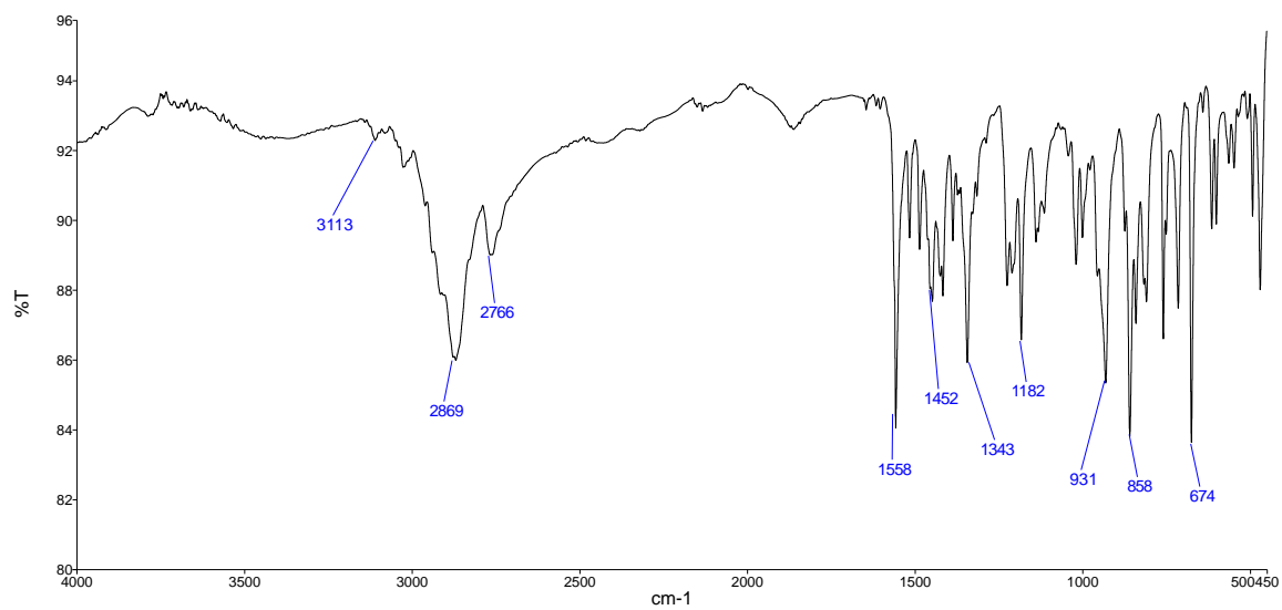
Figure S6. FT-IR spectrum of 3
