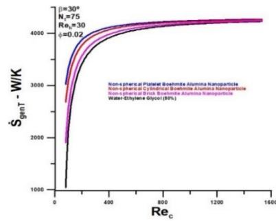
Figure 10. Thermal entropy generation rate versus Reynolds number with volume fraction of nanoparticles equal 2.0% as parameters
